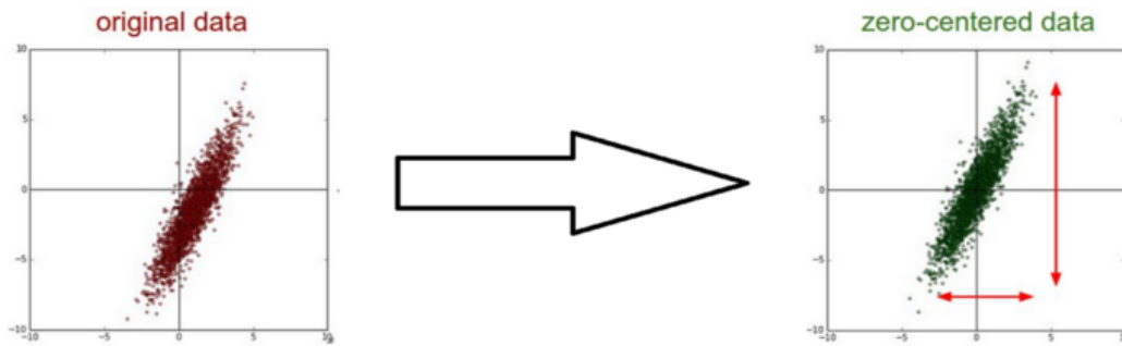
Figure 17: Mean-subtraction (Zero centering the data)(source: http://cs231n.stanford.edu/ )
