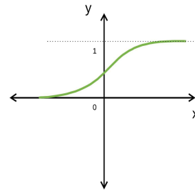
Figure 11: Sigmoid
