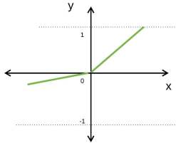
Figure 14: Leaky ReLU
