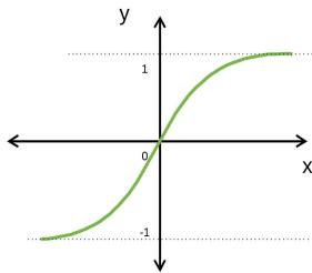
Figure 12: Tanh
