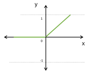
Figure 13: ReLU
