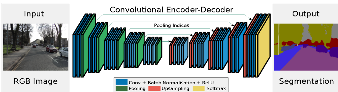
Figure 43: End-to-end model of SegNet[2].
