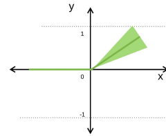
Figure 15: Noisy ReLU
