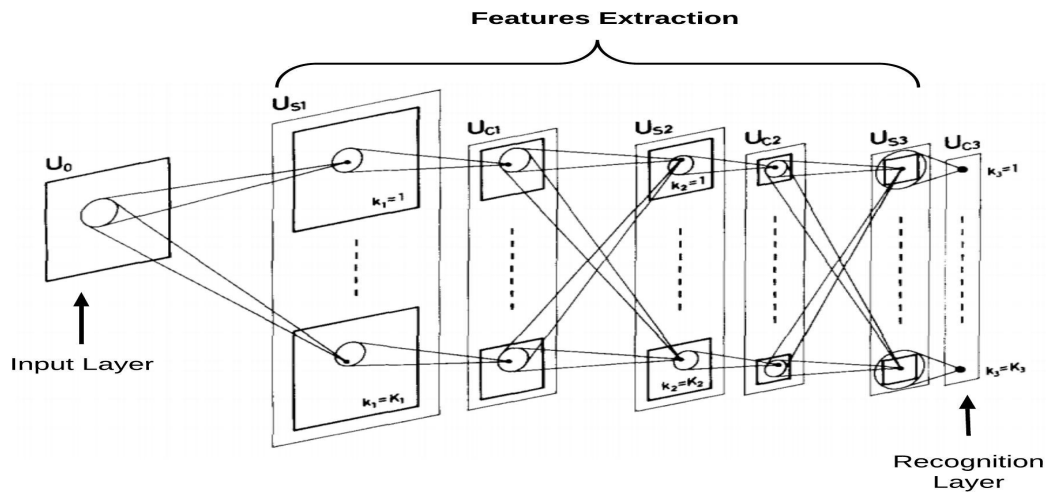
Figure 1: Schematic diagram illustrating the interconnections between layers in the neocognitron, Kunihiko Fukushima [7].
