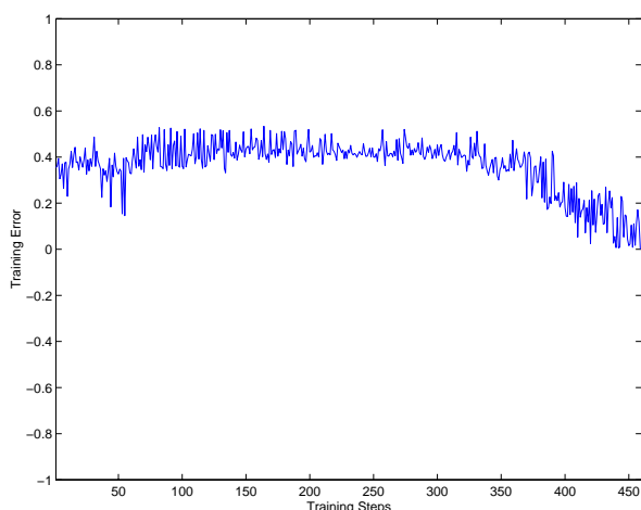
Fig. 8. Training Error
