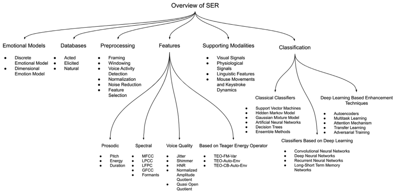
Fig. 1. An overview of speech emotion recognition systems. The recognition requirements flow from left to right. The emotions are embedded in the databases on the far left, and they are extracted at the far right end of the figure.
