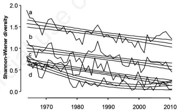
Fig. 2. Mean values of the Shannon-Wiener diversity index with a trend and 95% confidence limits. a, total zooplankton; b, Rotifera; c, Cladocera; d, Copepoda.
